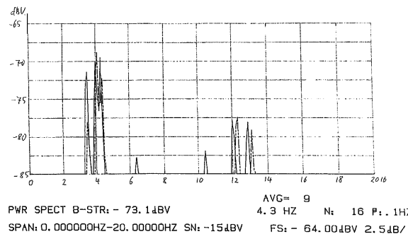
Fig.13: Spectra in the ELF-region („ Vitakur“, 4 repetitions)
