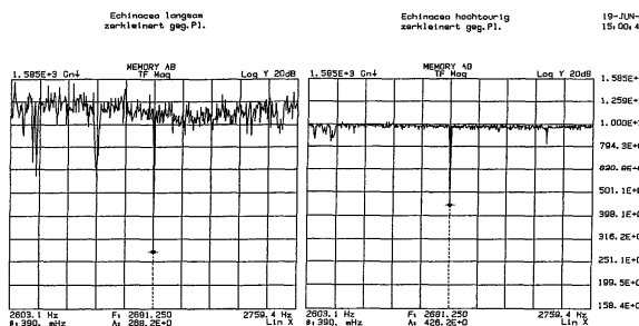
Fig. 9: spectrum of slowly grinded echinacea (left) and with high speed (right)
