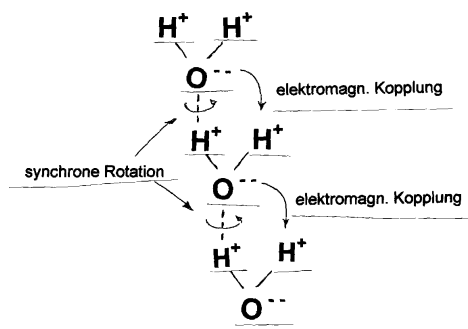
Fig. 3: the two phase model of (\text{H}_2\text{O})_n
