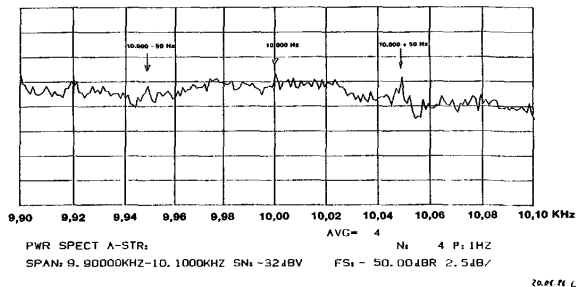
Fig.11: storage of 10 kHz in water
